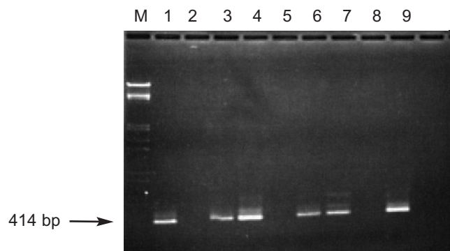
Figure 2. Nested PCR amplification of the 414-bp fragment. M= marker, 1= F. arundinacea E+, 2= F. arundinacea E-, 3= FaTsh 1 isolate, 4= F. pratensis E+, 5= F. pratensis E-, 6= FpGan 1 isolate, 7= F. arundinacea E+ 8= F. arundinacea E-, 9= FaFn 1 isolate.
