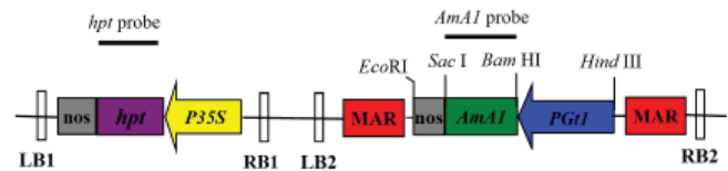
Figure 1. The T-DNA structure of binary plasmid vectors pCDMAR AmAl - hpt . hpt = hygromycin phosphotransferase; P35S = promoter of cauliflower mosaic virus; nos = 3' signal of nopaline synthase; MAR = tobacco Rb 7 matrix attachment regions; AmAl = Amaranth albumin gene; pGt1 = rice glutelin Gt1 promoter; LB1 , RB1 = left and right borders of the first T-DNA region; LB2 , RB2 = left and right borders of the second T-DNA region. As indicated in the figure, a full length fragment of hpt or AmAl coding region was used as a probe.
