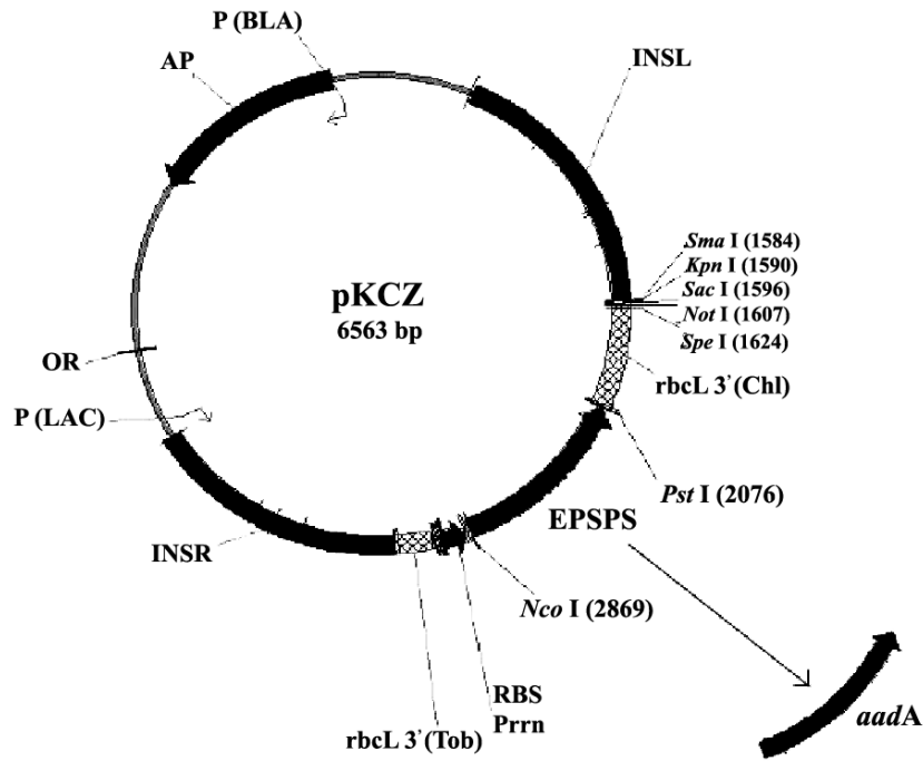
Figure 1. Substitution of the aadA gene with the mutated epsps synthase using the Nco I and Pst I digestion sites. epsps synthase integrates into the plastid genome through homologous recombination. INSL and INSR are identical to the flanking regions of the insertion site. For more details see materials and methods section.
